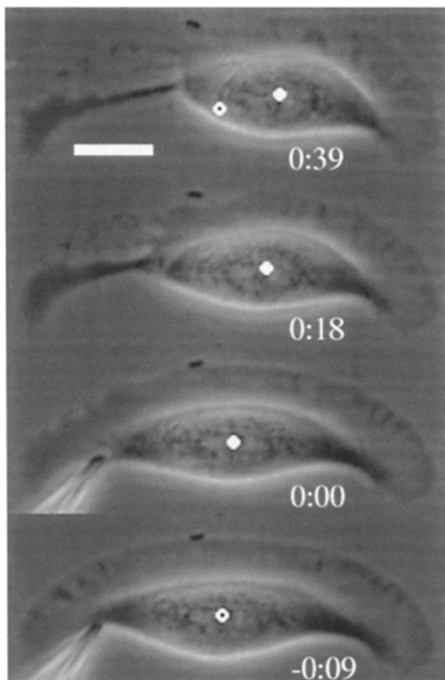
Figure 9. Traumatic microinjection at the end of the cell body (0:00) causes local disruption of the cytoskeleton and retraction of the cell body toward the opposite side. (White spots) Center of the cell body; (white spot with black point) position before injection, at time -0:09. Bar, 10 \mu m.
