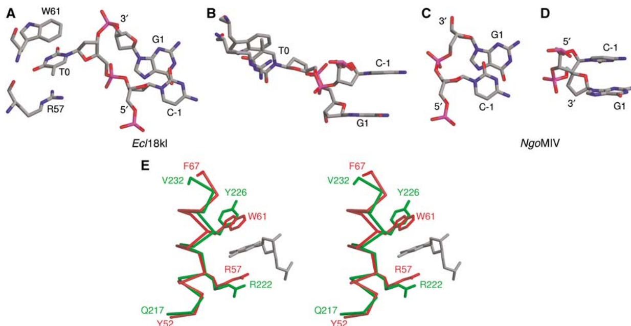
Figure 7 Close-up view of the central nucleotides in the Ec 18kI-DNA and Ngo MIV-DNA complexes. (A, B) Three central nucleotides (−1, 0, +1 according to Figure 1) of one strand in the recognition sequence of Ec 18kI are shown in stick representation and CPK colors. Note that there is still uncertainty whether the extruded bases have syn- or anti-conformation. Arg57 and Trp61 residues of Ec 18kI that sandwich the extruded base are shown in stick representation. (C, D) Two central nucleotides (−1, +1 according to Figure 1) in one strand of the Ngo MIV recognition sequence are shown in stick representation and CPK colors. (B) and (D) differ from (A) and (C) by 90°-rotations about the horizontal axis. (E) Structural conservation of the binding pocket for the flipped nucleotide in Ec 18kI and Eco RII (shown in red and green colors, respectively). Superposition between the Ec 18kI and Eco RII protomers reveals that Arg57 and Trp61 residues sandwiching the extruded base spatially coincide with Arg222 and Tyr226 of Eco RII. A flipped out base in the Ec 18kI-DNA complex is shown in gray, for one of the two possible binding modes of the DNA.
