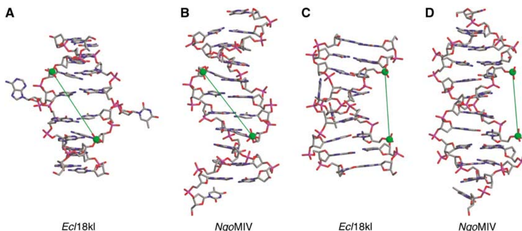
Figure 6 DNA conformation. DNA in complexes with Ec 18kI (A, C) and Ngo MIV (B, D) is shown in stick representation. Views in (C) and (D) differ from (A) and (B) by a 90° rotation around the vertical axis. The central nucleotide pair is flipped out of the DNA helix in Ec 18kI-DNA complex (A, C). The electron density for the central bases is averaged due to the two possible binding modes. The flipped out nucleotide is shown in one of the possible conformations, since there is still an uncertainty whether the flipped nucleotides have syn- or anti-conformation. Phosphorous atoms at scissile phosphates are shown as green spheres. The distance between these phosphorous atoms is 17.2 Å in both Ec 18kI-DNA and Ngo MIV-DNA complexes.
