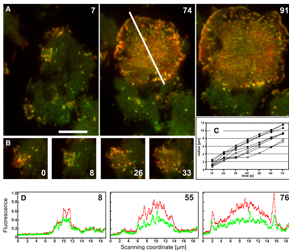
FIGURE 6 Wave propagation without SCAR. The expression of mCherry-LimEΔ and GFP-Arp3 in SCAR-null cells shows waves propagating with normal speed and their association with the Arp2/3 complex. (A) Merged images of mRFP-LimEΔ (red) and GFP-Arp3 (green) in three stages of an expanding wave. (B) Sequence illustrating origin of this wave from an area of dense and dynamic actin and Arp2/3 assembly. Time is indicated in seconds. Bar for A and B, 5 \mu m. (C) Velocity of wave expansion in SCAR-null cells. Distance of the actin front from the origin of two waves from an area of dense and dynamic actin and Arp2/3 assembly. Time is indicated in seconds. Bar for A and B, 5 \mu m. (D) Three scans of fluorescence intensities (in arbitrary units) along the line indicated in A. Red, mCherry-LimEΔ; green, GFP-Arp3. Numbers indicate seconds in accord with A and B. On the left of each panel the wave propagates toward the top in A, on the right toward the bottom.
