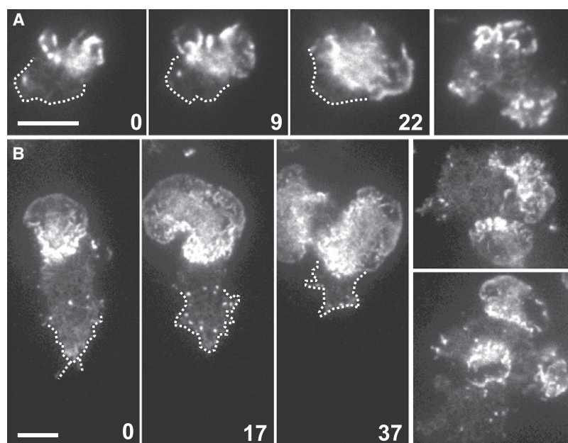
FIGURE 5 Independence of wave formation from signal transduction through heterotrimeric G-proteins. (A) Parent strain DH1. (B) G \beta -null mutant LW6 (27), both expressing LimEΔ-GFP. Time series on the left show the evolution of single waves; the one in B is split into two. Numbers indicate seconds. Panels on the right exemplify cells with two or three waves. Outside the waves the actin network in the cell cortex is distinguishable. The actin patches in this area are mostly involved in clathrin-dependent endocytosis (51). The two time series are typical in showing retraction of this area when the wave expands, as indicated by dotted lines. Bars, 10 \mu m.
