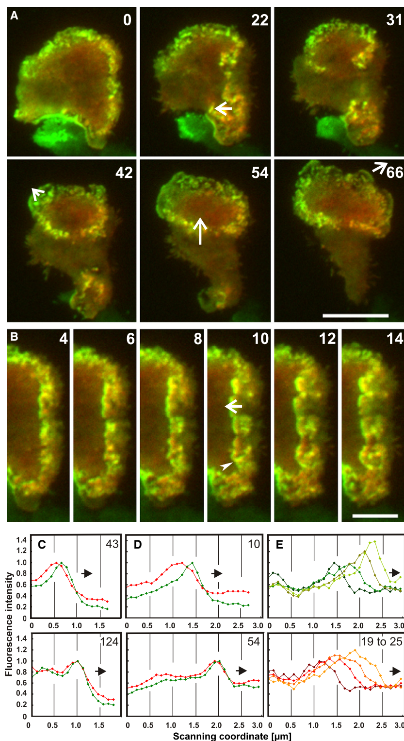
FIGURE 2 MyoB at the front of waves and their substructures. The GFP-MyoB label (green) is superimposed on the mRFP-LimEΔ label for filamentous actin (red). Cells recovering from latrunculin A treatment were recorded by TIRF microscopy (A,B) and fluorescence profiles quantified by line scans (C–E). (A) A wave showing irregular orientation of substructures during its reversal from collapsing to expanding. (B) A wave front in the same cell propagating from the right to the left and showing partitioning into ensembles led by MyoB. (Arrowhead in the 10-s frame; see also Movie S5 for substructure dynamics). Time is indicated in seconds after the first frame in A. Bars, 10 \mu\text{m} in A and 5 \mu\text{m} in B. (C) Two scans through waves that expand the cell border. (D) Two scans through retracting portions of waves that propagate on the substrate-attached cell surface. (E) Separate propagation of a substructure as indicated in the 22-s frame of A, plotted at 2-s intervals. (Top panel: dark to light green for MyB. Bottom panel: dark to light red for the actin label). Arrows in A and B indicate local direction of wave propagation and position of the scans in C–E. Numbers within panels C–E are seconds after the first frame in A; corresponding scan positions are indicated in A and B. (Position of the 124-s scan is indicated in the 66-s panel of A.) In C–E, the directions of wave propagation are plotted toward the right as indicated by arrows.
