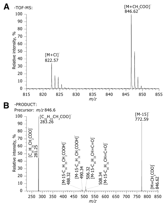
Fig. 1. A: TOF MS spectrum of synthetic 18:1/18:0-phosphatidylcholine (PC) standard in chloroform-methanol (1:2) containing 5 mM ammonium acetate (note that the standard contained \sim 19\% of the isomeric 18:0/18:1-PC, Table 1). PC was detected as anions of acetate and chloride adducts at m/z 846.62 and m/z 822.57, respectively. B: MS/MS spectrum of the acetate adduct at m/z 846.62 acquired at collision energy 40 eV. Peaks at m/z 772.59, 283.26, and 281.25 correspond to the fragment ion of demethylated PC ( [M - 15]^- ) and acyl anions of stearic and oleic acid, respectively. Low abundant fragments were produced by the loss of fatty acids as ketenes [M - 15 - C_{16}H_{31}CH=C=O]^- ( m/z 508.34) and [M - 15 - C_{16}H_{33}CH=C=O]^- ( m/z 506.32) and by neutral loss of free fatty acids [M - 15 - C_{16}H_{31}CH_2COOH]^- ( m/z 490.34) and [M - 15 - C_{16}H_{33}CH_2COOH]^- ( m/z 488.32).
