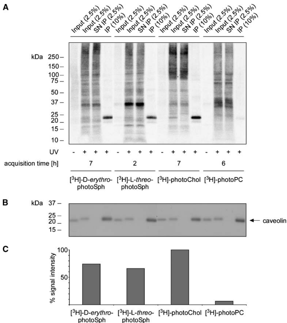
Fig. 7. Caveolin-1 interacts with cholesterol and sphingolipids. CHO cells were labeled for 20 h with 200 \mu\text{Ci} of [^3\text{H}]\text{-D-erythro-photoSph} , [^3\text{H}]\text{-L-threo-photoSph} , M \beta CD-complexed [^3\text{H}]\text{photoChol} , or [^3\text{H}]\text{choline}/50 \mu\text{M} 10-ASA. After UV irradiation, cells were subjected to immunoprecipitation using an anti-caveolin antibody. Samples of input (+/- UV irradiation), supernatant (SN), and pellet of immunoprecipitation (IP) were separated by SDS-PAGE and transferred to PVDF membranes. A: Radioactively labeled proteins were visualized by digital autoradiography, with acquisition times as indicated. B: Western blot analysis using the anti-caveolin antibody. C: Quantitation of immunoprecipitated radioactivity. The values are given as percentages compared with the sample with highest radioactivity.
