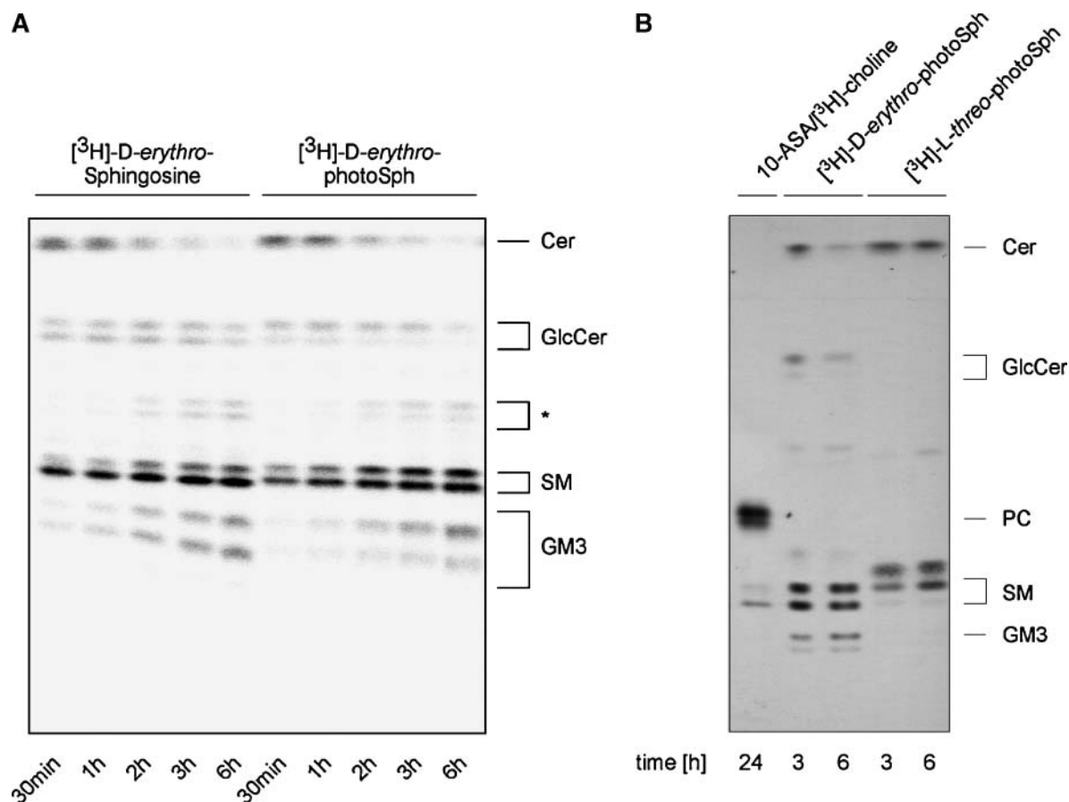
Fig. 3. Comparison of sphingolipid labeling using different lipid precursors. A: A 3 cm dish of CHO cells was labeled with 0.1 \mu\text{M} [ ^3\text{H} ]D-erythro-photoSph or [ ^3\text{H} ]D-erythro-sphingosine (4 \mu\text{Ci}/2 ml). Lipids were extracted as described and analyzed by TLC (solvent system: chloroform-methanol-water, 65:25:4, v/v/v) and digital autoradiography (β-Imager). The asterisk indicates that lipid comigrates with phosphoethanolamine Cer standard. B: A 10 cm dish of CHO cells was labeled with 1 \mu\text{M} (200 \mu\text{Ci}/10 ml) of either D-erythro- or L-threo-photoSph or with 50 \mu\text{M} 10-azido-stearic acid (10-ASA) per 100 \mu\text{Ci}/10 ml choline chloride for different times. Lipids were resolved by TLC using chloroform-methanol-water (65:25:4, v/v/v) as the solvent system. The TLC plate was sprayed with Amplify Fluorographic Reagent (NAMP-100; Amersham) and exposed to Hyperfilm™ (HP79NA; Amersham Biosciences) at -80^\circ\text{C} . A quantity of 0.05 \mu\text{Ci} was applied per lane. For details, see Experimental Procedures.
