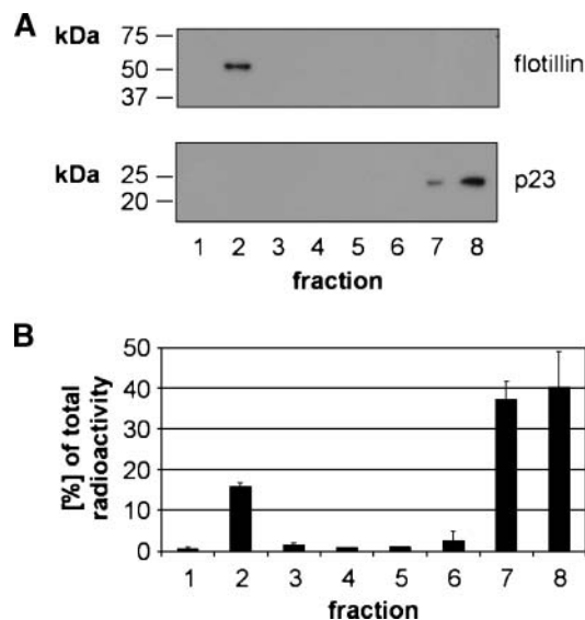
Fig. 5. Photolabile sphingolipids partition into detergent-resistant membranes (DRMs). A total of 1 \times 10^7 CHO cells (two 10 cm dishes) were grown in the presence of 1 \mu\text{M} (200 \mu\text{Ci}/10 ml and dish) [ ^3\text{H} ] D-erythro -photoSph for 6 h. After extraction with cold Triton X-100 at 4°C, samples were subjected to Optiprep density centrifugation as described. Gradients were fractionated from top to bottom into eight fractions. A: Gradient fractions were analyzed for DRM (flotillin) and detergent-soluble membranes (p23) by Western blotting. B: The radioactivity of each fraction was measured, and values are given as percentage of total radioactivity for all gradient fractions ( n = 2 ). Error bars indicate \pm SD.
