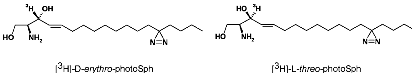
Fig. 1. Structures of [^3\text{H}]\text{-D-erythro-photoSph} (photoSph) and [^3\text{H}]\text{-L-threo-photoSph} . For details, see text.
