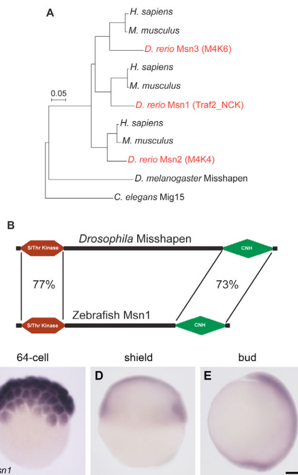
Fig. 2. msn1 encodes a zebrafish orthologue of Drosophila Misshapen and is expressed during gastrulation. (A) Phylogenetic analysis of zebrafish homologues (Msn1-3) of Drosophila Misshapen. The scale bar indicates point mutations per site. Msn1 is most closely related to human and mouse Traf2_NCK (Traf2 and NCK interacting kinase). (B) Protein domain comparison of zebrafish Msn1 and Drosophila Misshapen. Percentage amino acid identity between conserved N-terminal Ser/Thr kinase and C-terminal CNH (citron homology) domains is indicated. (C-E) msn1 mRNA expression during early cell division gastrulation stages. In situ hybridization of wild-type embryos at 64-cell (C), shield (D) and bud stages (E). Dorsal is to the right in D and E. Scale bar in E: 100 μm for C-E.
