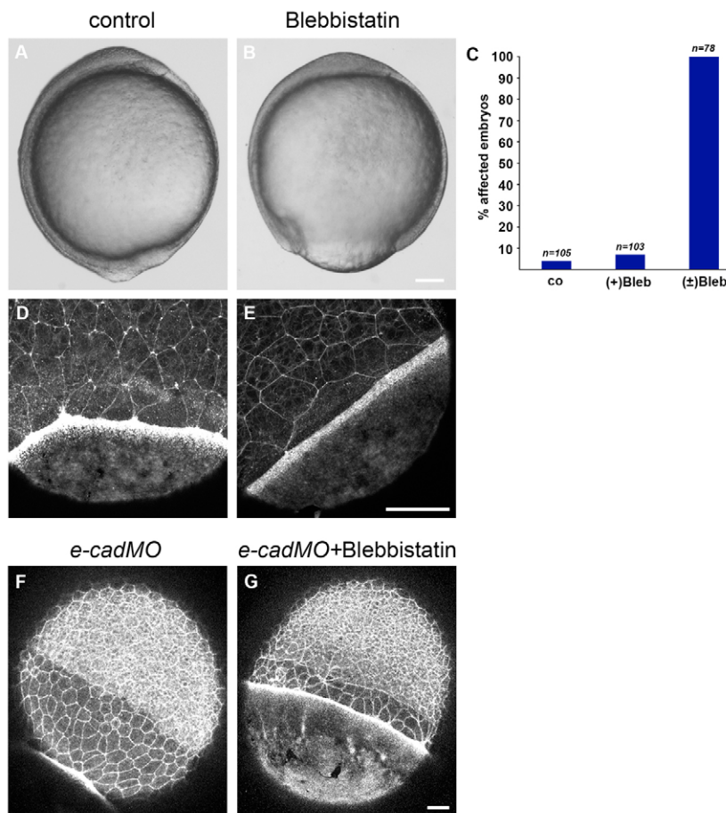
Fig. 5. Treatment with the myosin 2 inhibitor blebbistatin decreases actin recruitment in the YSL and slows the rate of EVL epiboly.
