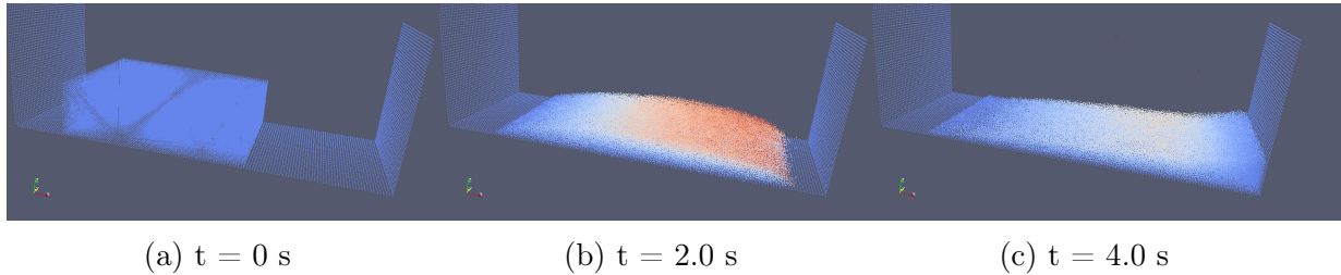
Figure 5: Visualization of PPME simulation results of an avalanche down an inclined plane. The panels show the particles at the indicated times. Color from blue to red indicates the x -component of the velocity of the particles.
