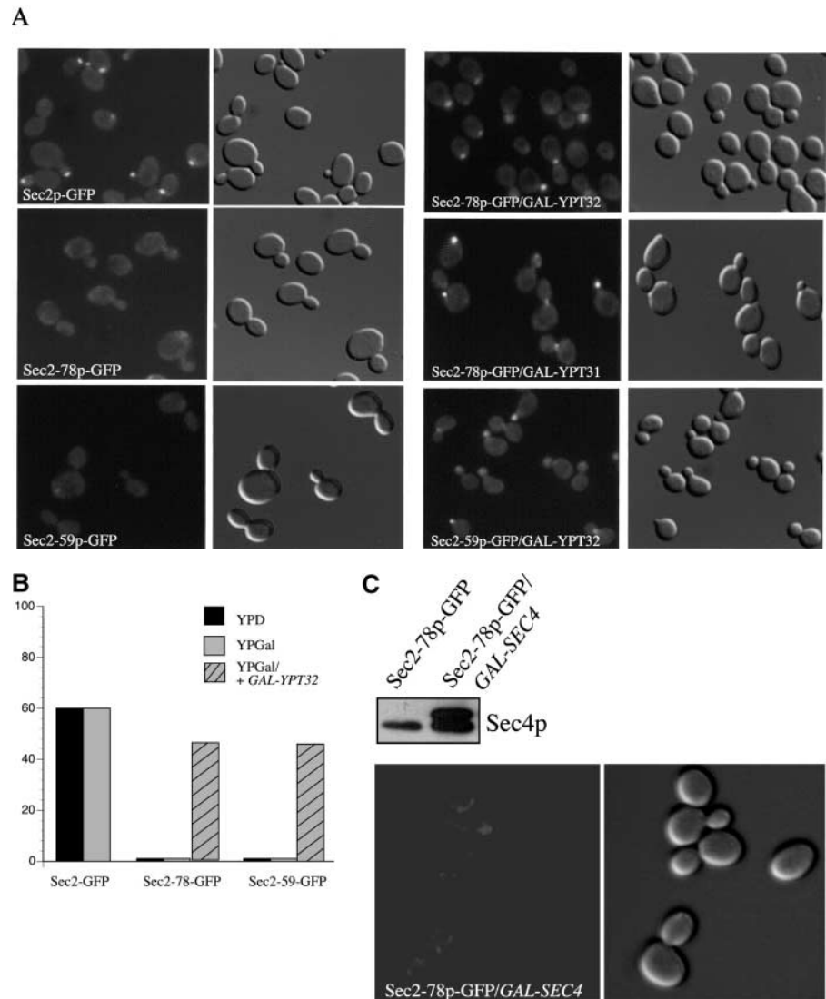
Figure 2. Overexpression of Ypt32p restores the localization of Sec2-78p-GFP and Sec2-59p-GFP. Yeast were grown from stationary cultures overnight at 25°C to log phase on YPGal. For GFP visualization, cells were harvested, fixed in methanol, permeabilized, washed with PBS, and directly observed. (A) Representative wild-type Sec2p-GFP (NY2146), Sec2-59p-GFP (NY2147), and Sec2-78p-GFP (NY2152) fields are shown. Sec2-78p-GFP/GAL-YPT32 (NY2429), Sec2-78p-GFP/GAL-YPT31 (NY2430), and Sec2-59p-GFP/GAL-YPT32 (NY2428) show restored localization of Sec2 proteins when grown on YPGal. (B) Approximately 100 cells were counted for each experiment and the percentage of cells showing bud tip and mother-daughter neck localization of Sec2p-GFP, Sec2-78p-GFP, and Sec2-59p-GFP. 60% of wild-type cells show polarized localization of Sec2p-GFP. Sec2-78p and Sec2-59p-GFP show <1% of localized protein. When Ypt32p is overproduced (YPGal), restored localization of Sec2 proteins is observed in 46% of cells. (C) Overexpression of Sec4p from the GAL promoter does not affect the localization of Sec2-78p-GFP (NY2446). Western blot was probed with \alpha Sec4p antibody.
