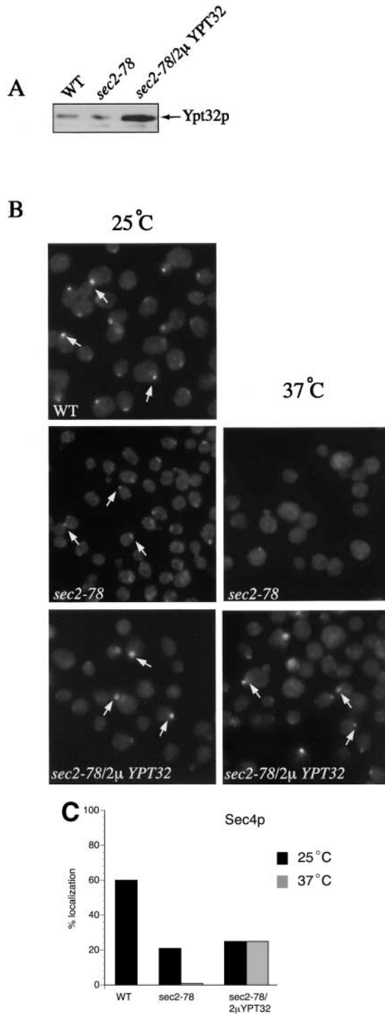
Figure 3. Ypt32p overexpression partially restores the localization of Sec4p. (A) For these experiments, sec2-78 cells (NY2179) were transformed with a 2μ URA3 plasmid overproducing YPT32 from the GPD promoter (NY2431). Overexpression was confirmed by Western blot probed with αYpt32p antibody. (B) For Sec4p immunofluorescence, cells were grown overnight in YPD at 25°C, shifted to 37°C for 2 h, fixed, and labeled with αSec4p antibody. At 25°C, wild-type (NY10), sec2-78 (NY2179), and sec2-78/2μYPT32 cells (NY 2431) show Sec4p staining preferentially at the bud tip and necks (arrows). In sec2-78 cells, diffuse staining is observed after a temperature shift to 37°C, but upon Ypt32p overexpression, localization of Sec4p is partially restored (arrows). (C) Approximately 100 cells were counted for each experiment and the percentage of cells showing bud tip and mother-daughter neck localization of
