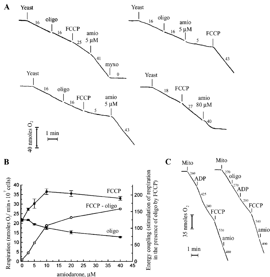
Figure 2. Effect of amiodarone on respiration of S. cerevisiae cells or mitochondria. Additions were as follows: (A and B) yeast, 0.6 \times 10^7 cells/ml; 10 \mu g/ml oligomycin (oligo); 1 \mu M FCCP; amiodarone (amio); 7 \mu M myxothiazol (myxo). (C) Yeast mitochondria (0.1 mg of protein/ml; mito); 150 \mu M ADP; 1 \mu g/ml oligomycin (oligo); 0.5 \mu M FCCP; 5 \mu M amiodarone. Numbers near the curves: nM O_2 /min \times 10^{-7} cells (A) or nM O_2 /min \times mg protein (C).
