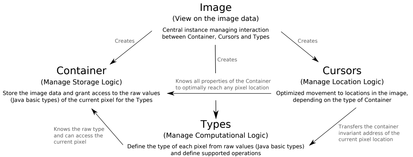
Figure 1. Visualization of the four major abstraction levels Type , Cursor , Container , and Image .
