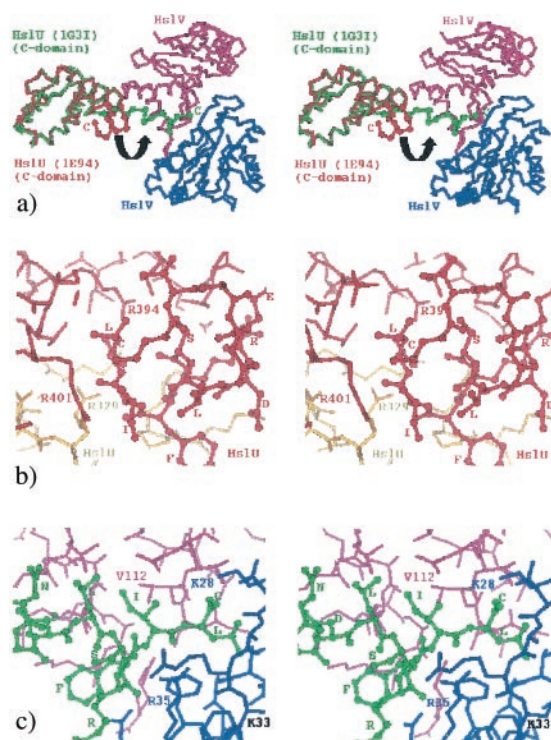
Fig. 1. (a) Stereo view ( C^\alpha -trace) of the superposition of the C domain of an HslU subunit (red) from the original E. coli HslVU complex (6) onto that of the H. influenzae HslU subunit (green) from its complex (19). Two HslV subunits (pink and blue) from the H. influenzae complex are also shown to illustrate the binding of the C-terminal segment of H. influenzae HslU to the pocket between the HslV subunits (indicated also by a black curved arrow). Color of the labels follows that of the respective subunits. Protein Data Bank codes are also indicated. (b) Stereo view of the close-up of the C-terminal residues of an E. coli HslU subunit (red) from the complex (6). The carboxylate of the terminal leucine residue forms salt bridges with R394 of the same subunit and with R329 of an adjacent (yellow) HslU subunit that is not illustrated in a for clarity. (c) Stereo view of the close-up of the C-terminal residues of an HslU subunit from the H. influenzae HslVU complex (19). Color coding is the same as in a. Residues of HslV that have been mutated in the present study in this region are indicated. K33, an essential residue of the catalytic apparatus of HslV is indicated in black.
