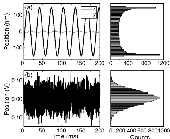
FIG. 1. Positions of the piezostage (a) and the trapped bead (b) for a stage moving sinusoidally with frequency f_{\text{drive}}=32 \text{ Hz} and amplitude A = 150 \text{ nm} in the x direction. (a) Left, time series of stage position; right, histogram of the x coordinate of the stage position. The sinusoidal movement results in two clear maxima. (b) Left, time series of the bead's x coordinate in volts, as given by the signal from the photodiode. The amplitude of the sinusoidal response is smaller than the amplitude of the thermal motion. Consequently the sinusoidal shape is masked by the Brownian motion of the bead, and the maxima associated with the sinusoid disappear in the histogram of visited positions (right).
