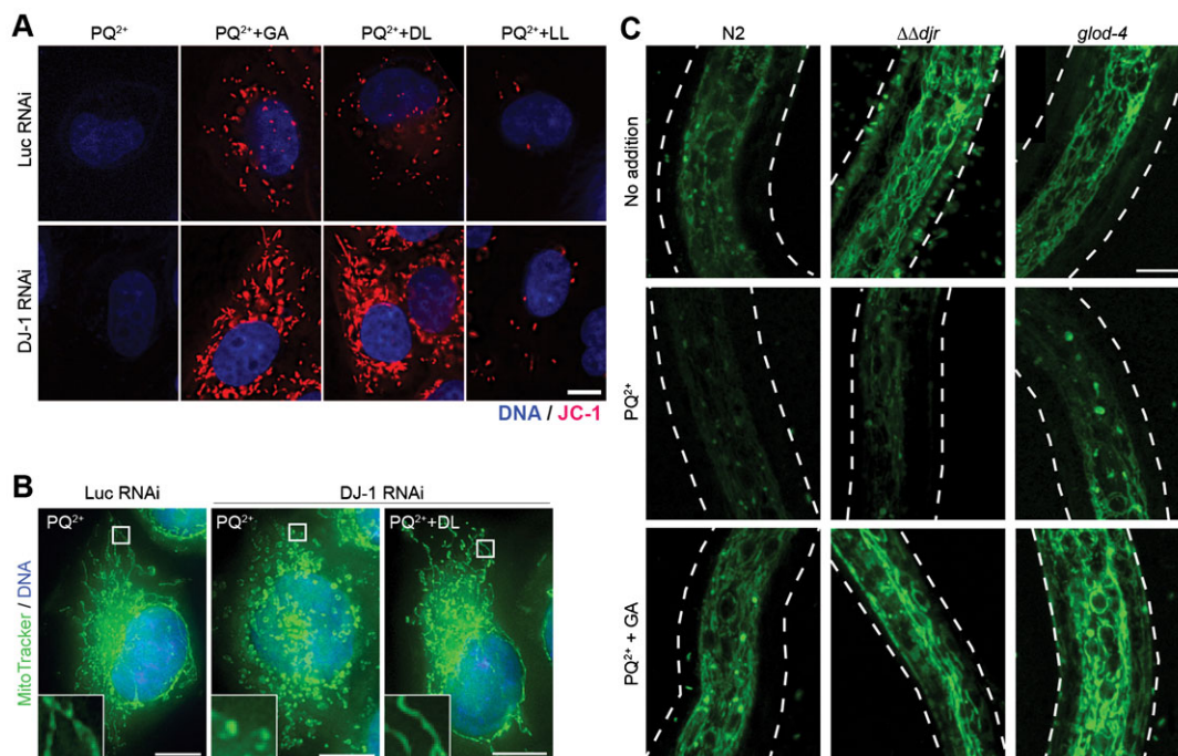
Fig. 3. Glycolate and D-lactate rescue the stress-induced mitochondrial defects. (A) JC-1 staining in live esiRNA-transfected HeLa cells treated with 50 \mu\text{M} paraquat ( \text{PQ}^{2+} ) and 1 mM of glycolate (GA), D-lactate (DL), and L-lactate (LL). Red, JC-1; blue, DNA. For merged images, see Fig. 4A. (B) Mitochondria of paraquat-treated HeLa cells. Green, MitoTracker; Blue, DNA. Inset, 4 \times magnification of the boxed area. (C) Mitochondria in worm glyoxalase mutant larvae. Wild type (N2), DJ-1 mutant ( \Delta\Delta djr ) and GLOD-4 mutant ( glod-4 ) were treated with \text{PQ}^{2+} with or without 10 mM GA, and stained with MitoTracker (green). Dashed lines show the outlines of larvae. Scale bars: 10 \mu\text{m} .
