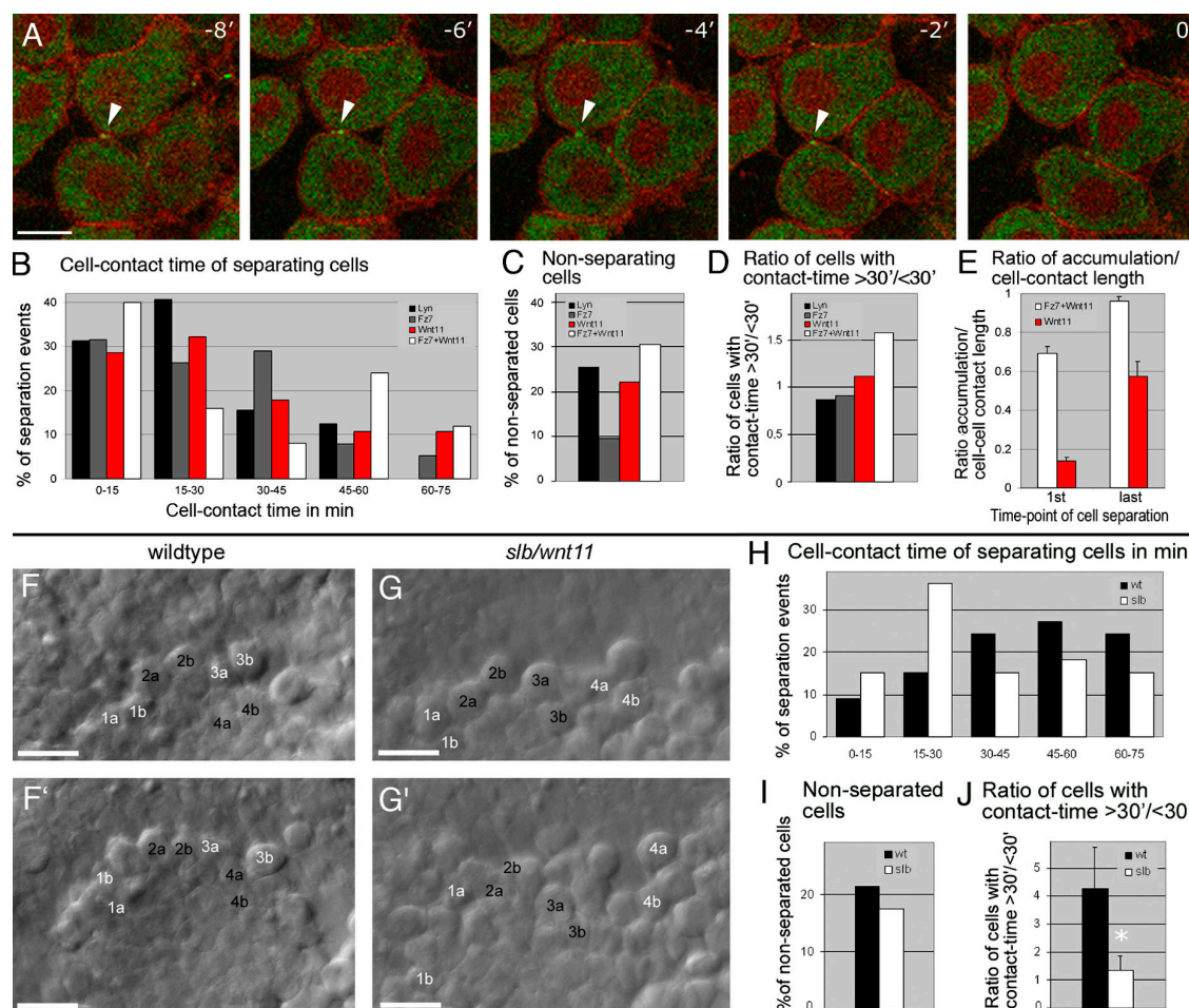
Figure 8. Wnt11 persist at cell contacts and is required for contact persistence. (A) Time series of separating hypoblast cells expressing a mix of 80 pg of wnt11-yfp and GPI-anchored rpf ( mem-rpf ) mRNA in shield-stage embryos (6 hpf). Wnt11-YFP (green) located in puncta at cell contacts (arrowheads) and remained until separation (Video 7). Time-series was obtained as in Fig. 5; time interval = 112 s. (B–E) Quantification of separation behavior of cells expressing Wnt11-YFP and mem-RFP (as in A, red) in animal pole assay (Video 8) compared with conditions described in Fig. 5 (G–H; Fz7-YFP + Wnt11, white; Lyn-YFP, black; Fz7-YFP, gray). (B) Relative distribution of contact times produced, as described for Fig. 5. Number of cells analyzed was as follows: 28 (Wnt11), 25 (Fz7 + Wnt11), 38 (Fz7), and 32 (Lyn) out of 4 videos per condition. (C) Percentage of cells not separating in 75 min. Number of cells analyzed was as follows: 36 (Wnt11), 36 (Fz7 + Wnt11), 42 (Fz7), and 43 (Lyn) out of 4 videos per condition. (D) Ratio of cells contacting for >30 min (including nonseparating cells)/cells separating for <30 min from start of video. Calculated from data in B and C. (E) Ratio of length of Wnt11 puncta or Fz7 accumulation/total contact length at the first video time point and the last time point before separation; number of cells analyzed was as follows: 20 (Wnt11) and 26 (Fz7 + Wnt11) out of 4 videos per condition. (F–G') Images of 3D time-lapse videos recorded for 75-min and 30-s time-intervals in wild-type (F and F', and Video 9) and slb/wnt11 (G and G', and Video 10) mutant embryos at late shield stage (7 hpf), using bright-field microscopy. "Head-on" view of the dorsal germ ring (shield) showing cells at the leading edge of the prechordal plate. Images shown are first (F and G) and last (F' and G') video time points. Numbers mark exemplary cells that separate (white) or remain in contact (black). (H) Relative distribution of cell contact times for separating wild-type and slb/wnt11 mutant prechordal plate progenitors (see Videos 9 and 10). Measured in 3D and presented as described for Fig. 5. Number of cells analyzed was as follows: 33 (wild type) and 37 ( slb/wnt11 ) out of 5 videos per condition. (I) Percentage of cells not separating in wild-type and slb/wnt11 mutant embryos in 75 min. Number of cells analyzed was as follows: 42 (wild type) and 44 ( slb/wnt11 ) out of 5 videos per condition. (J) Ratio of cells contacting >30 min (including nonseparating cells)/cells separating <30 min from start of video. Calculated from data in H and I. Asterisk represents the significant difference, with P < 0.05 . Error bars represent the SEM. Bars: (A) 10 \mu m; (F, F', G, and G') 50 \mu m. Videos 8–10 are available at http://www.jcb.org/cgi/content/full/jcb.200606017/DC1 .
